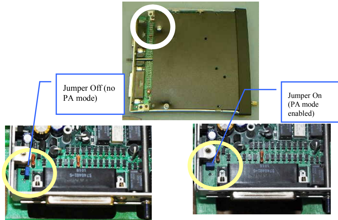
Figure 2-3 Jumper Location
